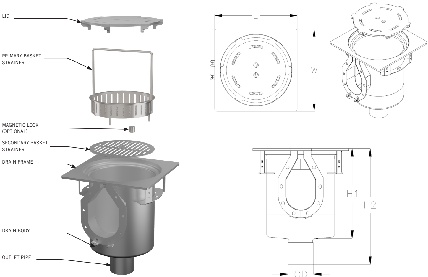
TYPICAL PROFILE OF A FOODSAFE SQUARE TOP CIRCULAR CATCH BASIN
